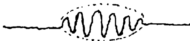
WAVE PACKET
